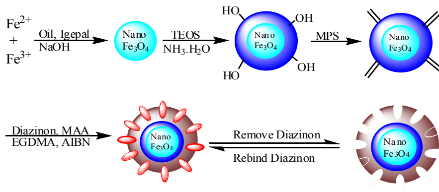
Figure 1. Scheme of preparation of \text{Fe}_3\text{O}_4@/\text{SiO}_2@/\text{MIP} .
