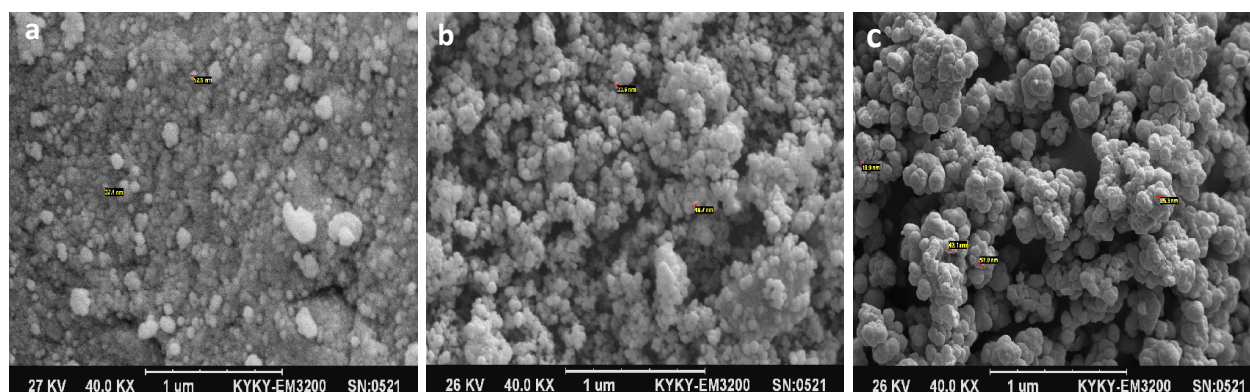
Figure 2. SEM images of \text{Fe}_3\text{O}_4 (a), \text{Fe}_3\text{O}_4@/\text{SiO}_2 (b), and \text{Fe}_3\text{O}_4@/\text{MIP} NPs (c).
